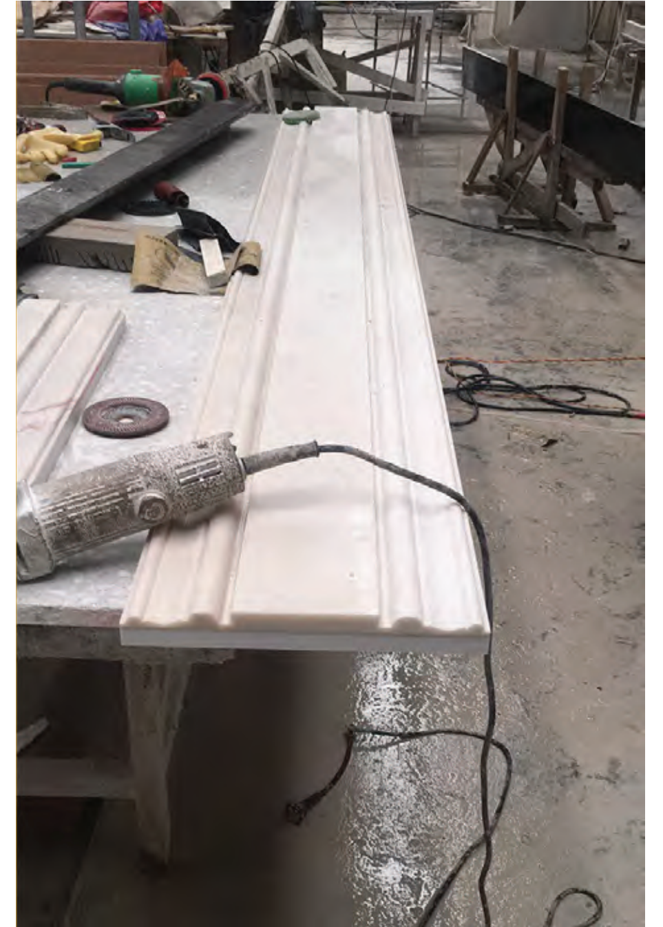
Process of Decoration lines
