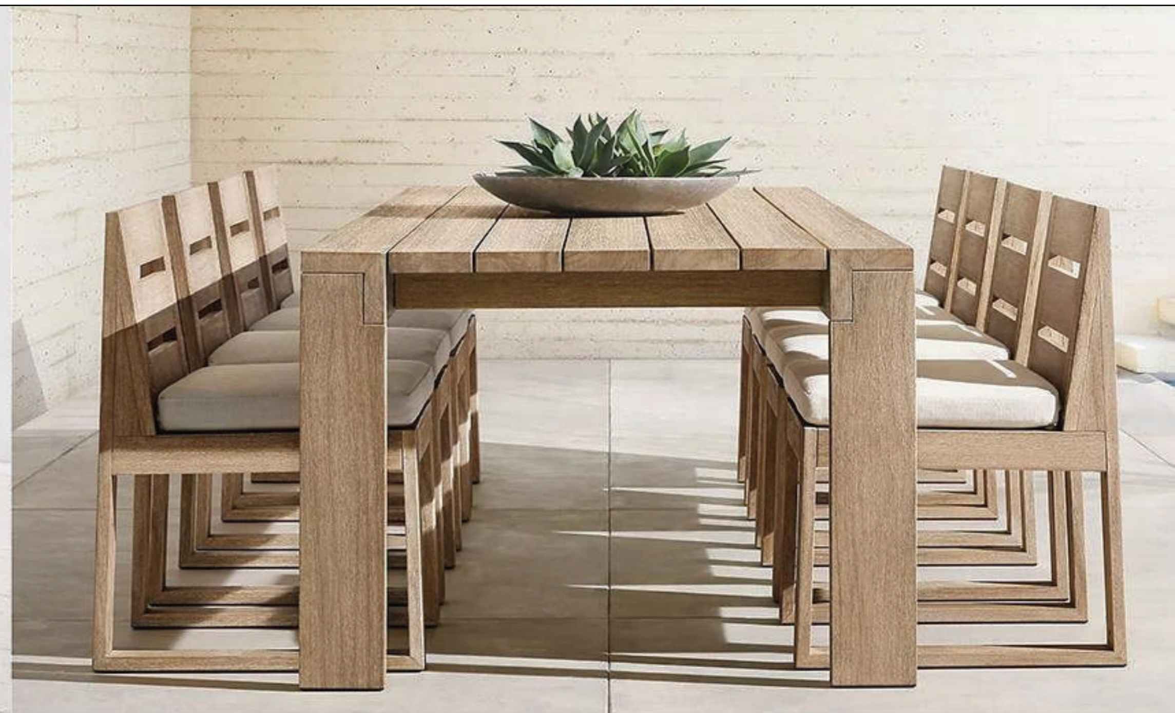
S616 CHAIR: D66×W50×H82CM SIDE CHAIR: D58×W50×H82CM TABLE: D180/240/300×W100×H75CM
