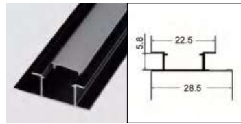
503 Light strip duplex line
