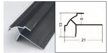
504 External corner line
