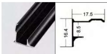
859 Inner corner line
