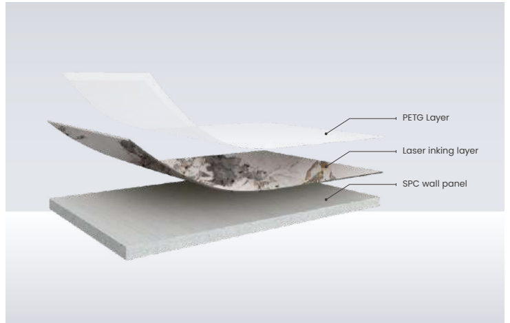
Product Structure Diagram
