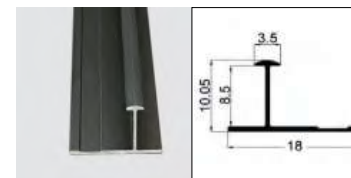
LT-A3 I-shaped line
