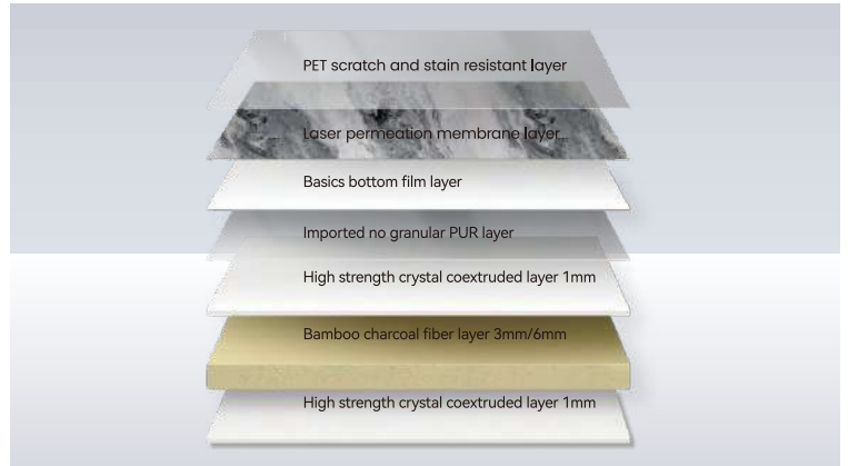
Product Structure Diagram
