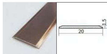
20 Flat metal strip
